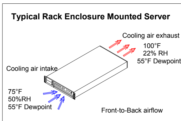
Figure 1 Server airflow and rack enclosure measuring point
