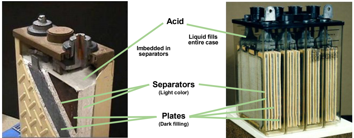
Figure 4 Typical lead-acid battery
